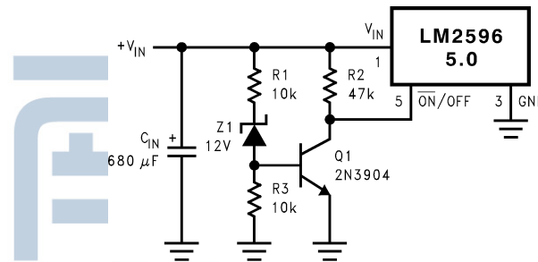
Figure 15. Undervoltage Lockout for Buck Regulator
